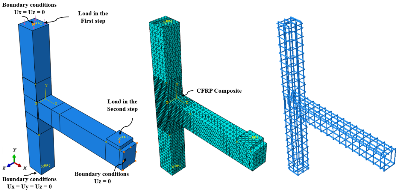
Fig. 9 Details and geometric representation of R2NS model
