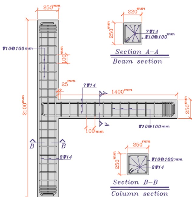
Fig. 1 NS and R2NS BCJ specimens – dimensions and reinforcement details [24]
