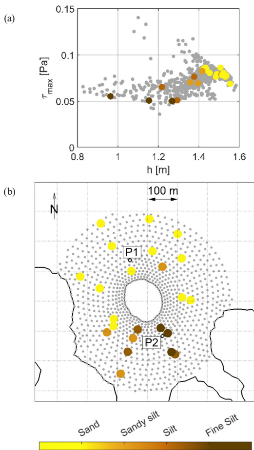
Fig. 7 (a) Scatter plot of the time-averaged \tau_{max,wc} v. water depth at the computational points in a 200 m diameter circle around the reed island for the actual bed, based on the simulations with the mean lake volume. (b) Horizontal layout of the computational points. Points where the bed material was surveyed are enlarged and colored according to the given scale
