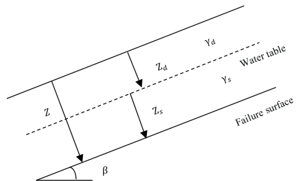
Fig. 6 The slope with translational slip
